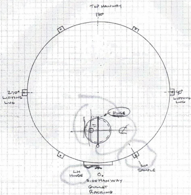
TRUE ORIENTATION OF FITTINGS
